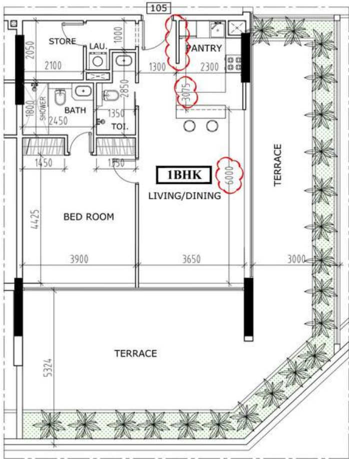
1BHK APARTMENT (TYPE-4)
